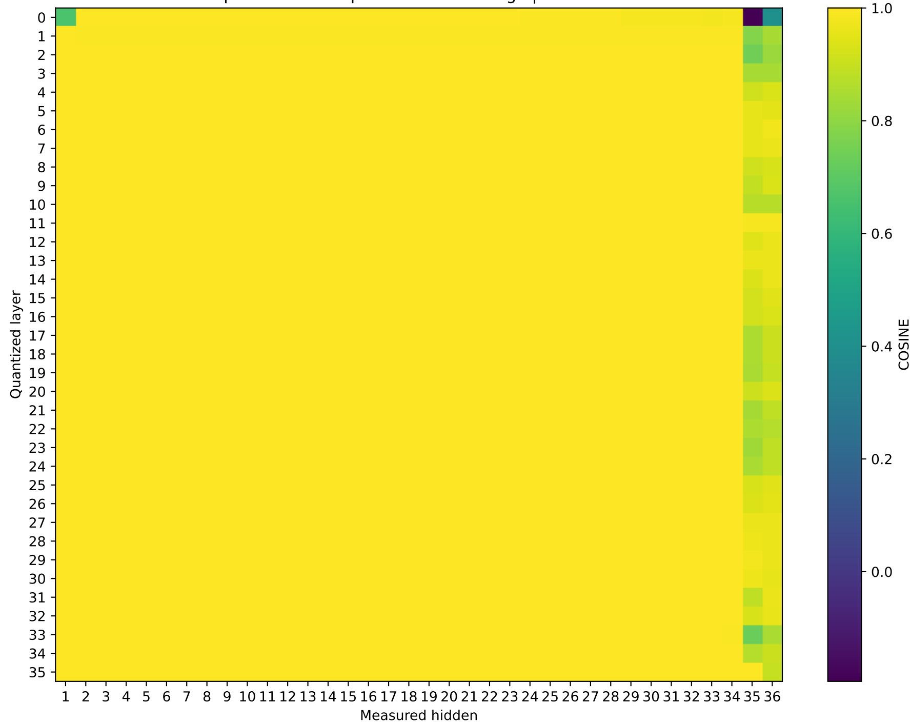
SmolLM3-3B Prompt 0: cos sim representation damage | float16 → int4
