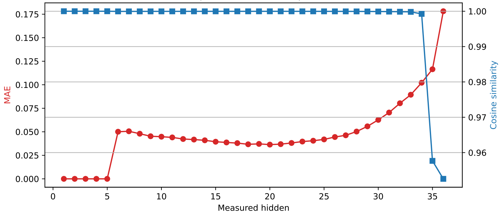
SmolLM3-3B | Quantized layer 5 | float16 \rightarrow int4
