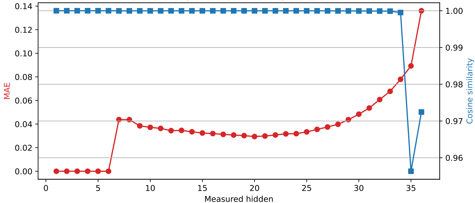
SmolLM3-3B | Quantized layer 6 | float16 \rightarrow int4
