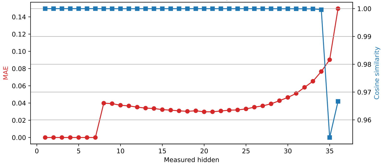
SmolLM3-3B | Quantized layer 7 | float16 → int4
