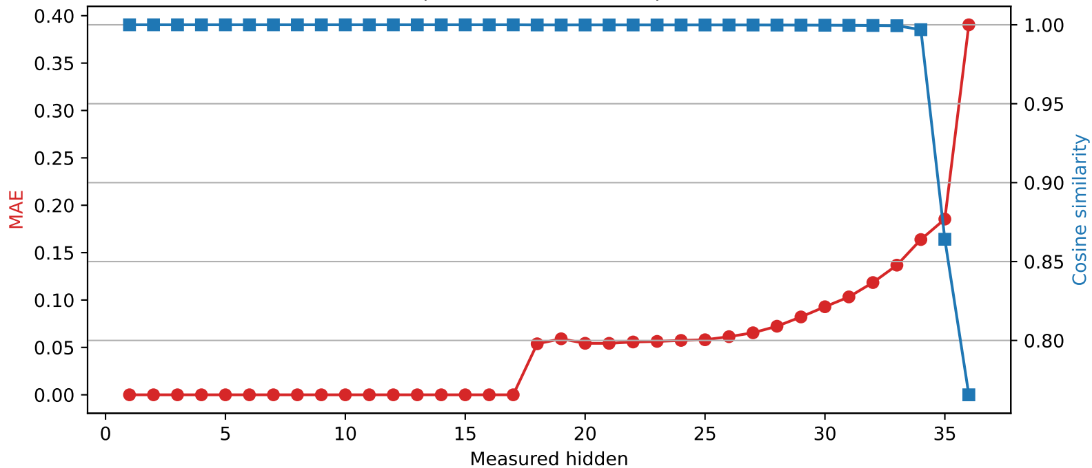
SmolLM3-3B | Quantized layer 17 | float16 → int4
