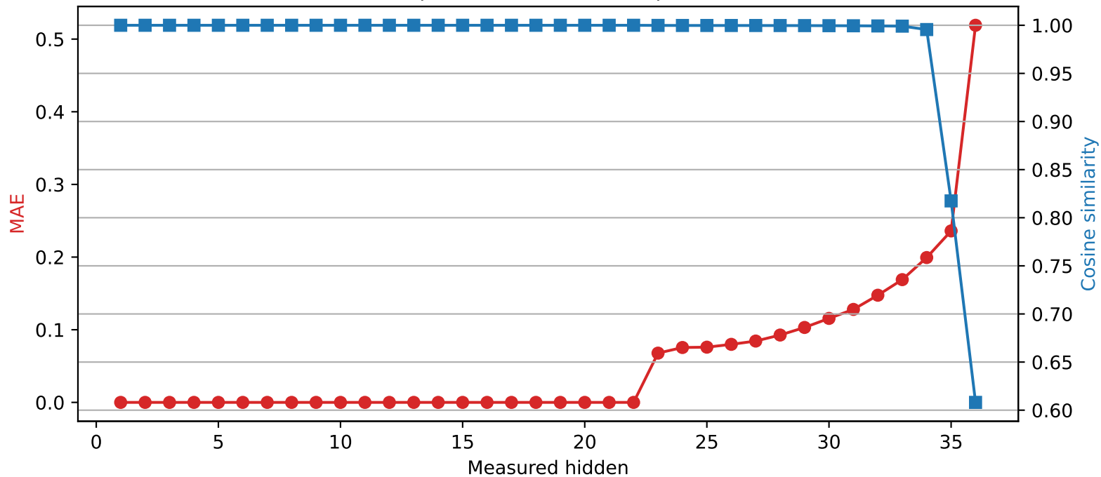
SmolLM3-3B | Quantized layer 22 | float16 → int4
