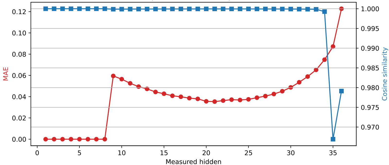
SmolLM3-3B | Quantized layer 8 | float16 \rightarrow int4
