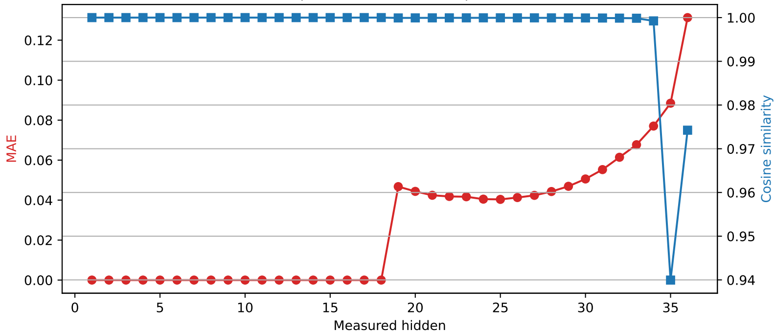
SmolLM3-3B | Quantized layer 18 | float16 → int4
