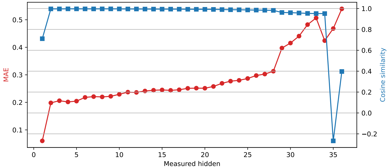
SmolLM3-3B | Quantized layer 0 | float16 \rightarrow int4
