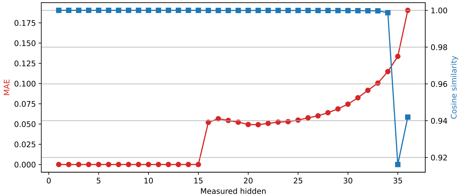
SmolLM3-3B | Quantized layer 15 | float16 \rightarrow int4
