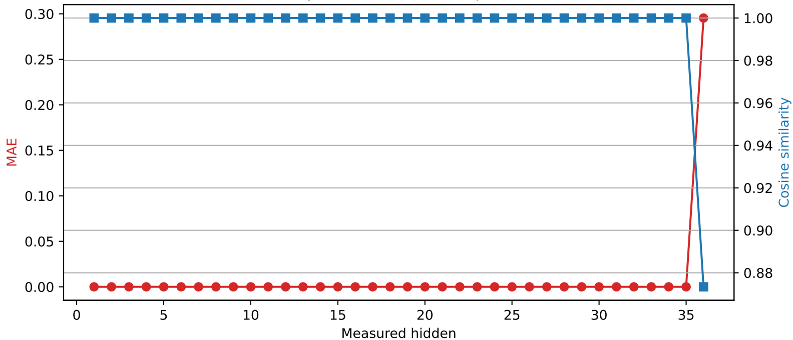
SmolLM3-3B | Quantized layer 35 | float16 → int4
