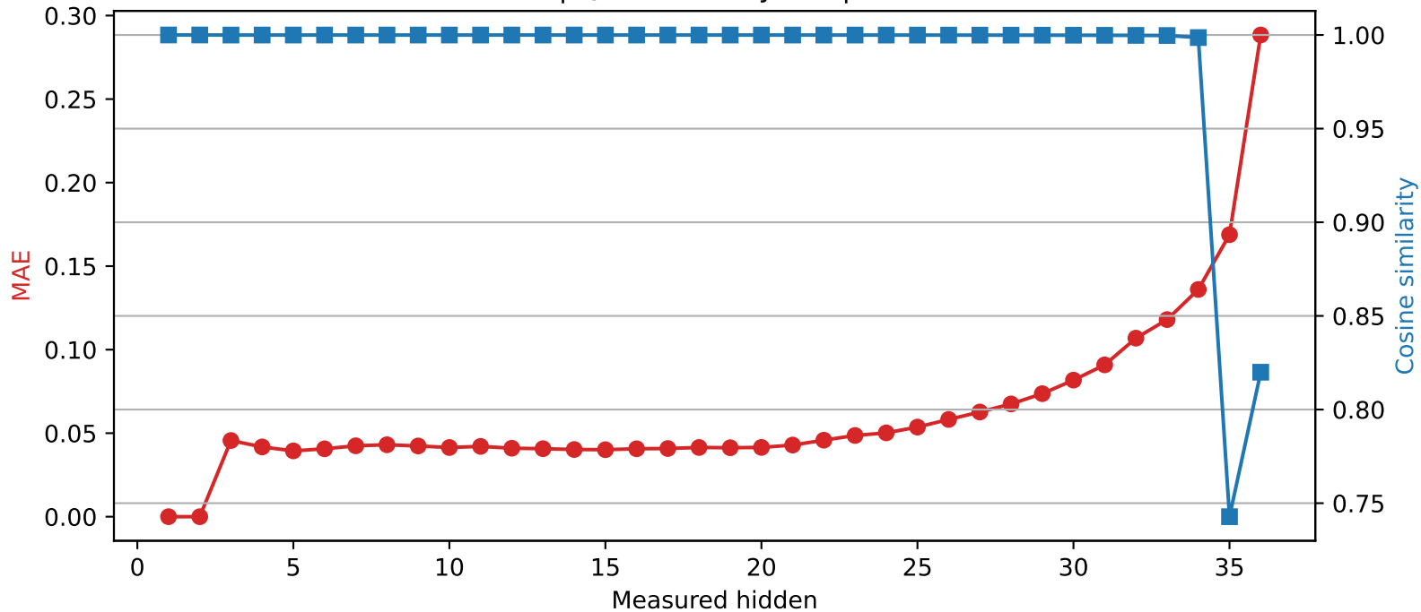
SmolLM3-3B | Quantized layer 2 | float32 \rightarrow int4
