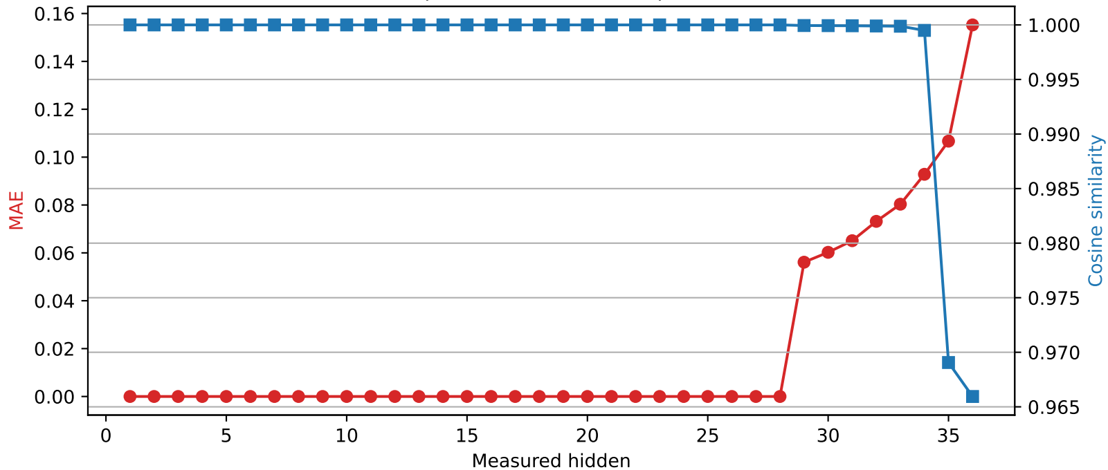
SmolLM3-3B | Quantized layer 28 | float32 → int4
