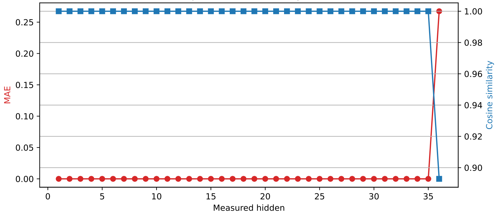
SmolLM3-3B | Quantized layer 35 | float32 → int4
