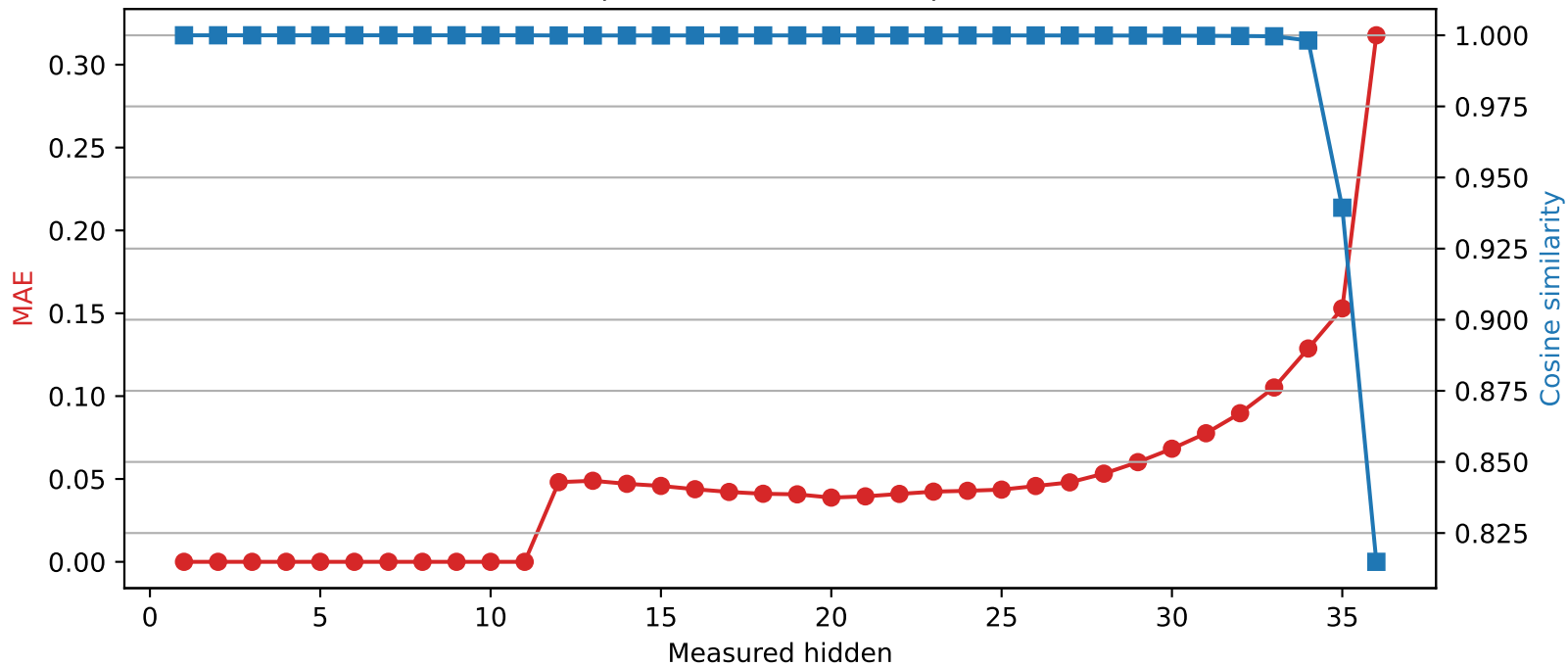
SmolLM3-3B | Quantized layer 11 | float32 → int4
