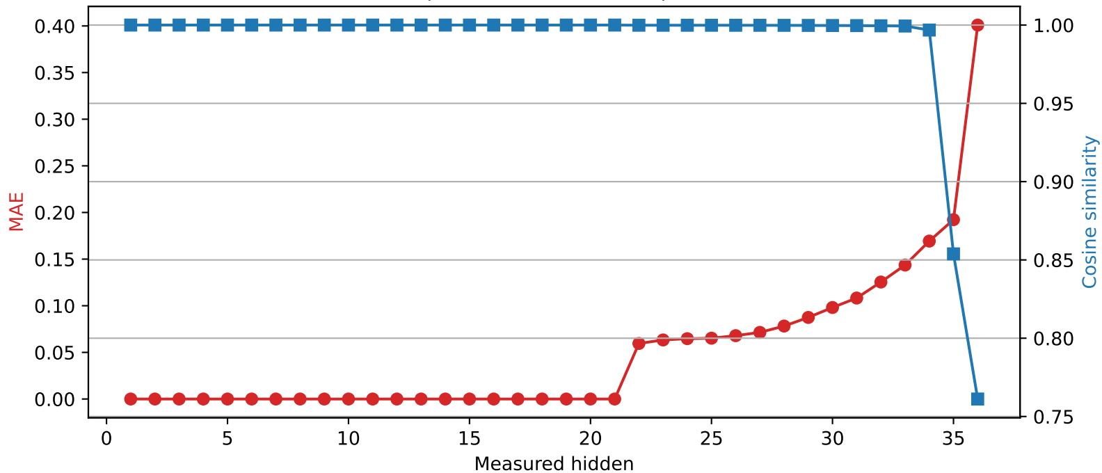
SmolLM3-3B | Quantized layer 21 | float32 → int4
