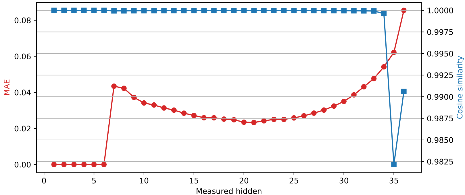
SmolLM3-3B | Quantized layer 6 | float32 \rightarrow int4
