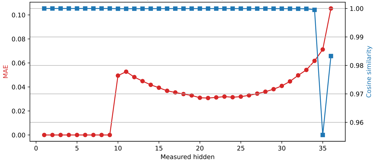
SmolLM3-3B | Quantized layer 9 | float32 \rightarrow int4
