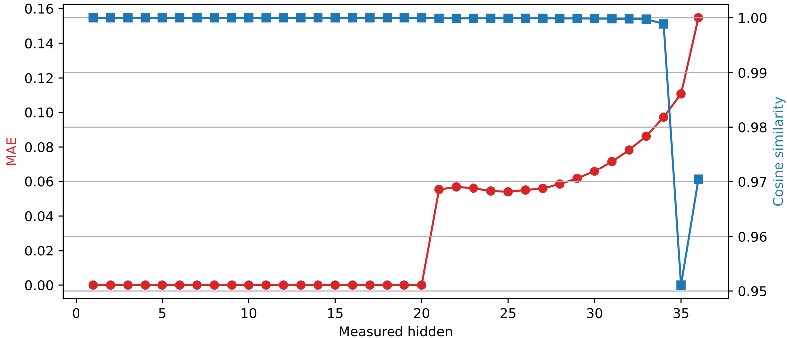
SmolLM3-3B | Quantized layer 20 | float32 → int4
