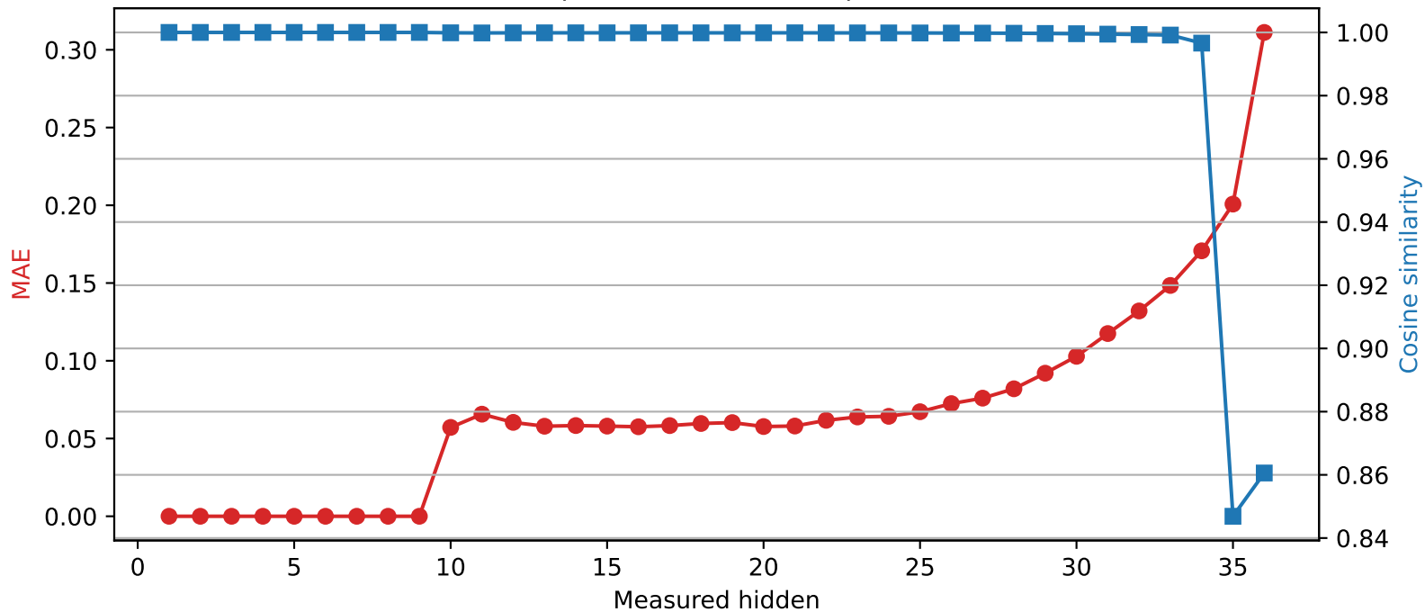
SmolLM3-3B | Quantized layer 9 | float32 → int4
