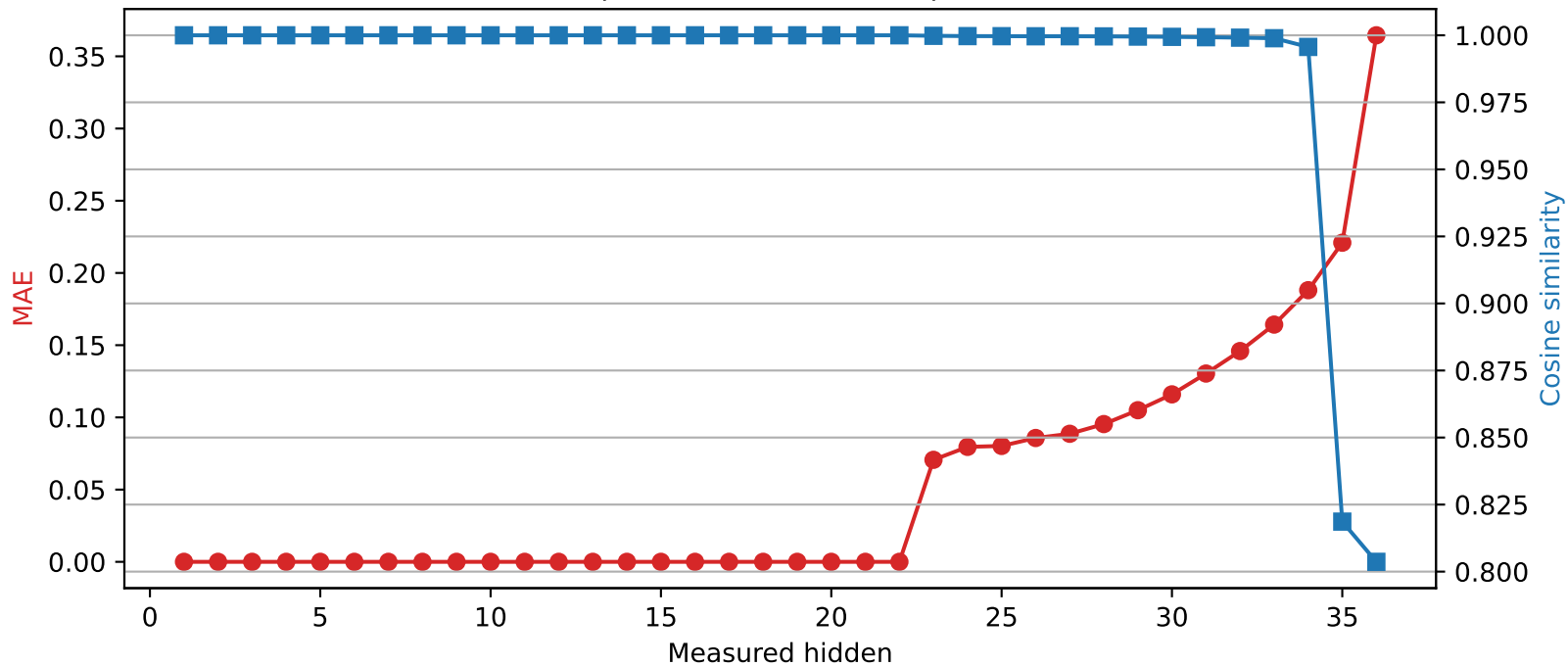
SmolLM3-3B | Quantized layer 22 | float32 → int4
