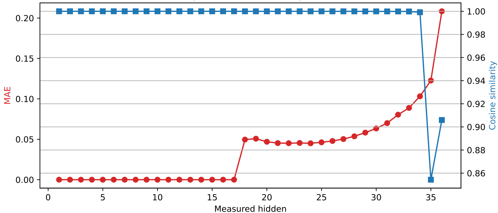
SmolLM3-3B | Quantized layer 17 | float64 → int4
