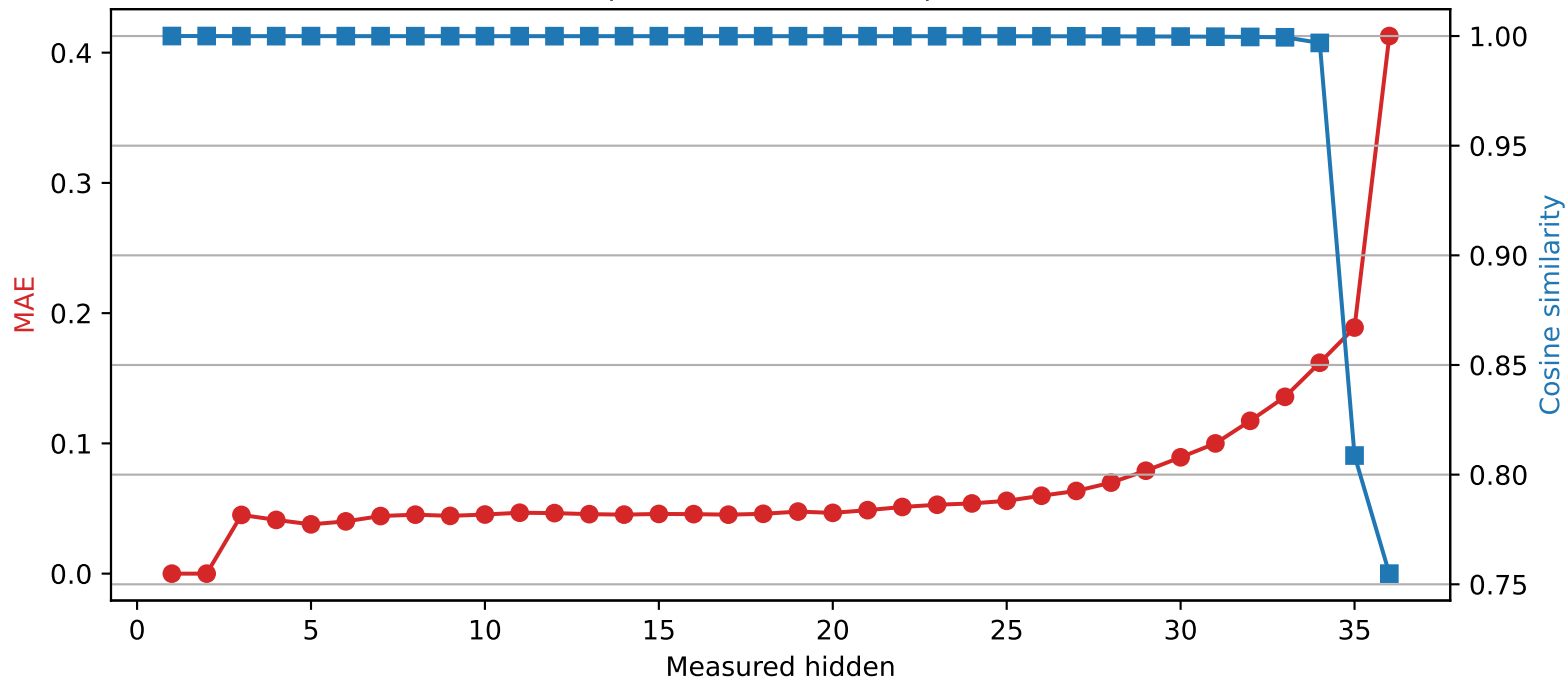
SmolLM3-3B | Quantized layer 2 | float64 → int4
