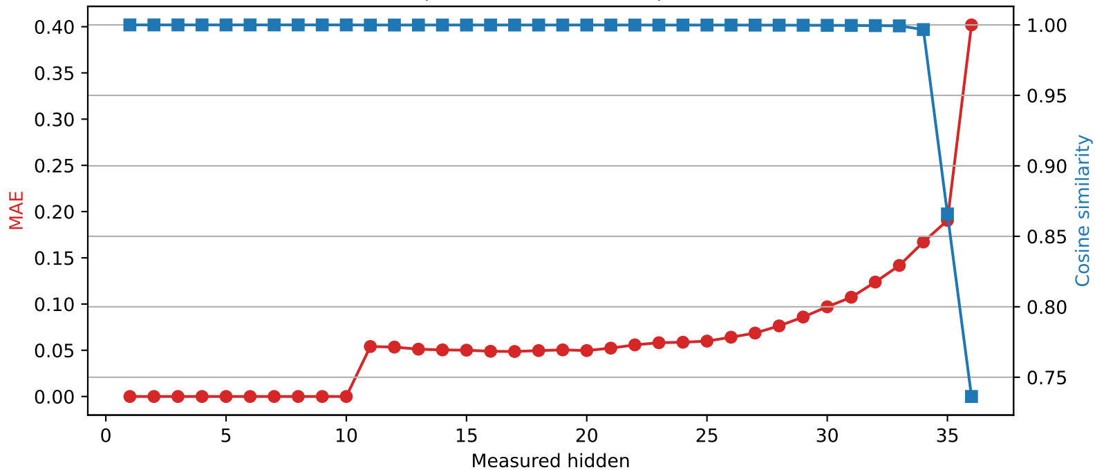
SmolLM3-3B | Quantized layer 10 | float64 → int4
