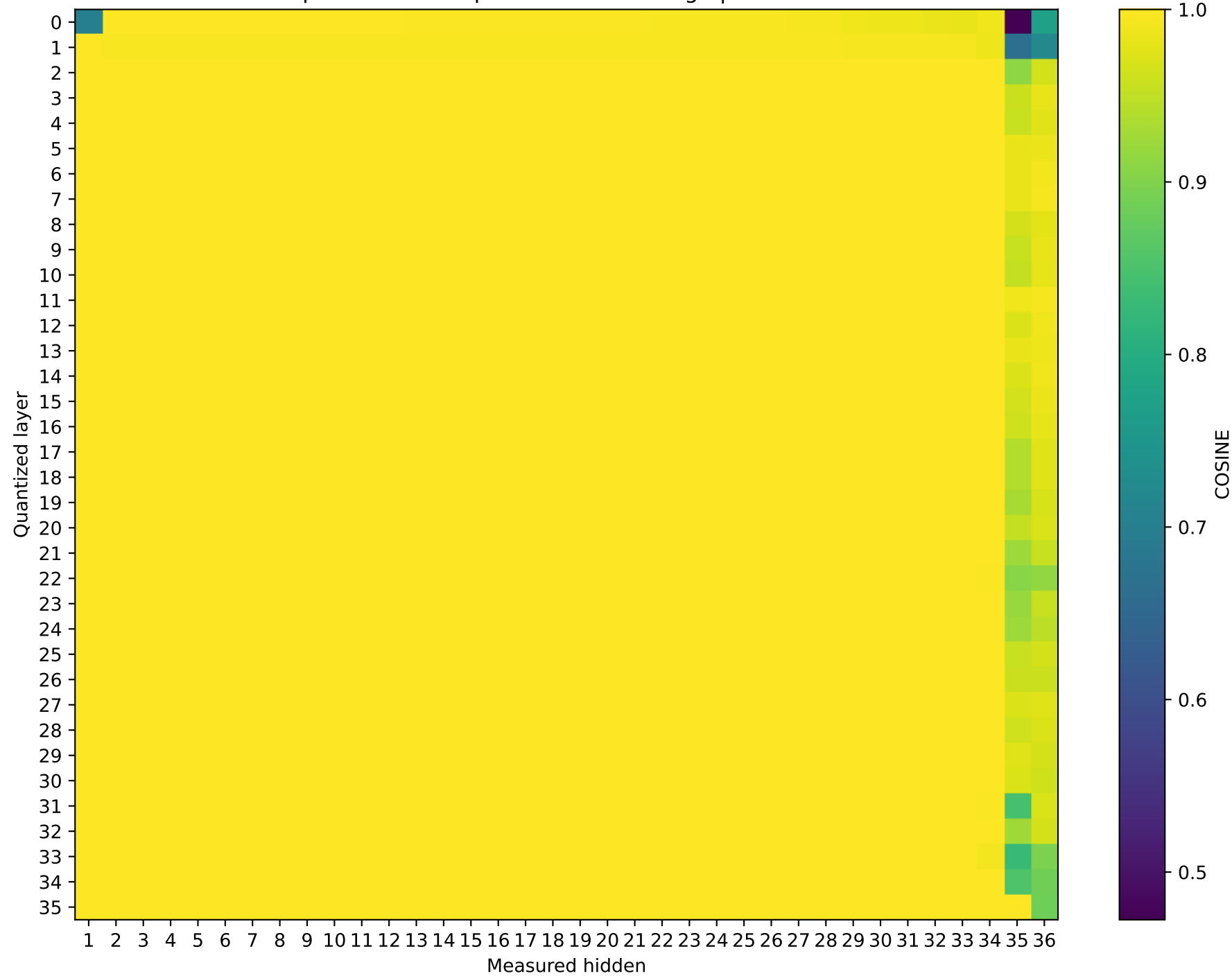
SmolLM3-3B Prompt 2: cos sim representation damage | float64 → int4
