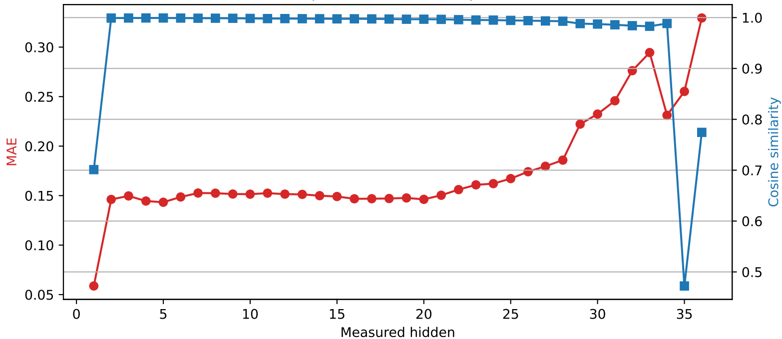
SmolLM3-3B | Quantized layer 0 | float64 → int4
