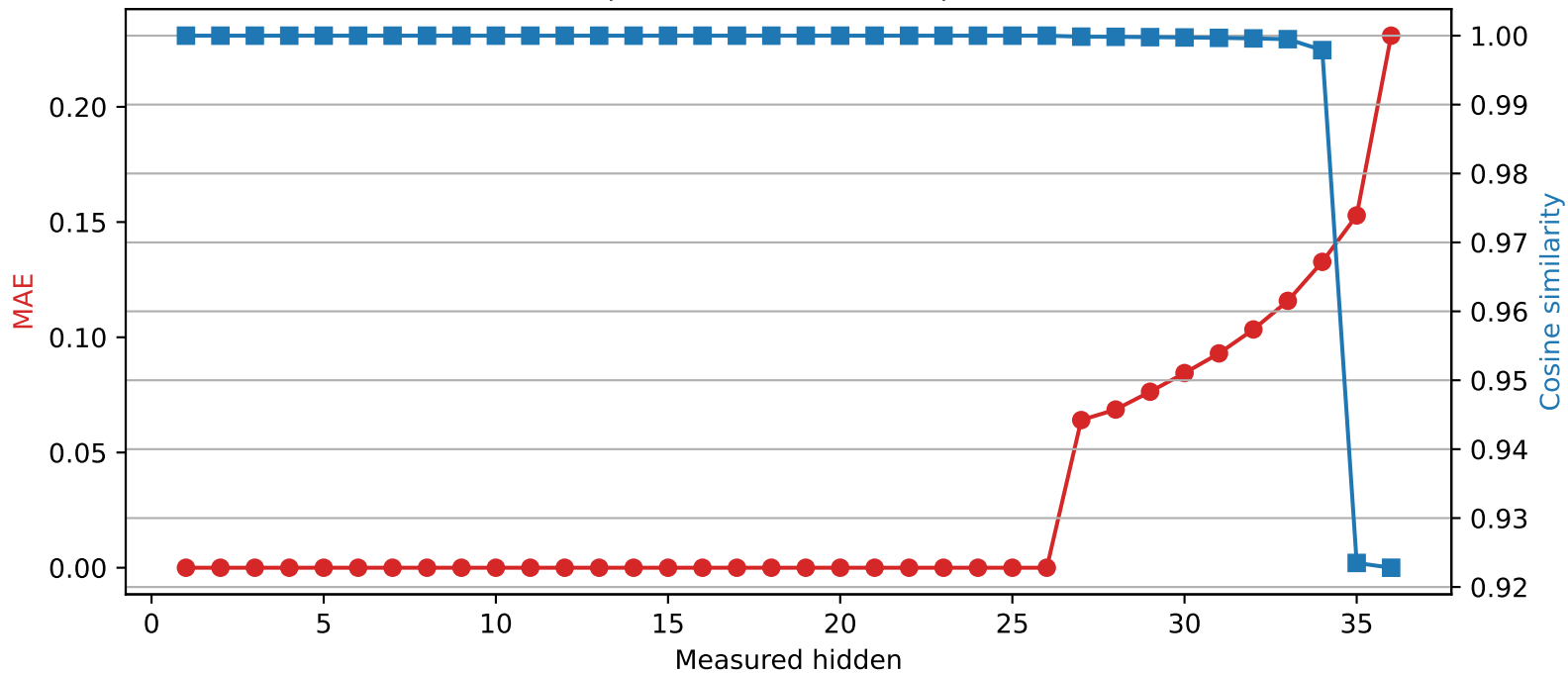
SmolLM3-3B | Quantized layer 26 | float64 \rightarrow int4
