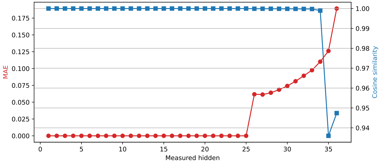
SmolLM3-3B | Quantized layer 25 | float64 → int4
