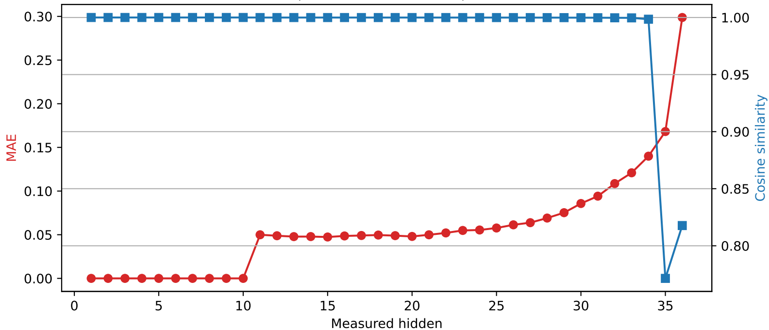
SmolLM3-3B | Quantized layer 10 | float16 \rightarrow int2
