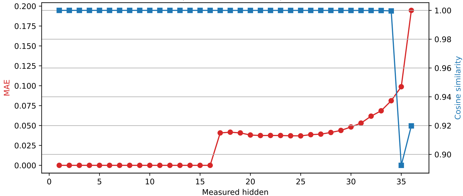
SmolLM3-3B | Quantized layer 16 | float16 \rightarrow int2
