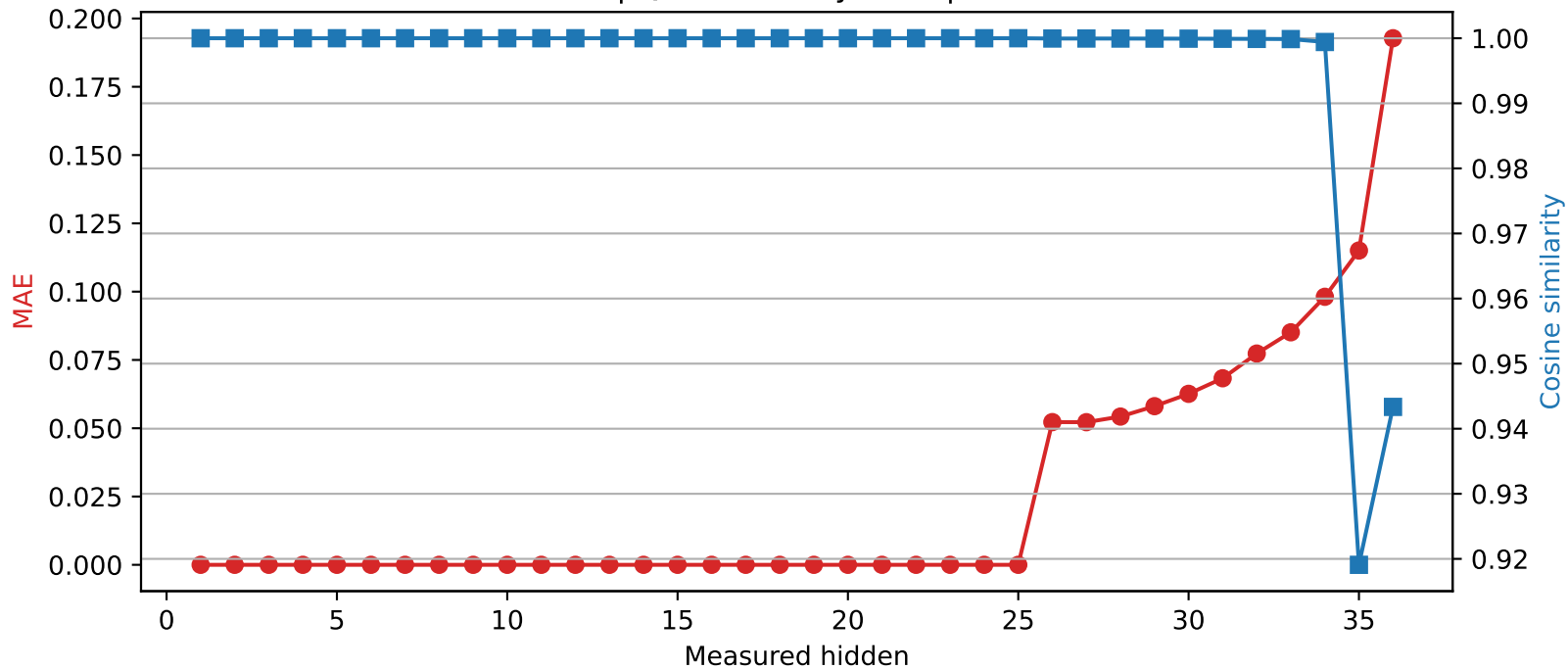
SmolLM3-3B | Quantized layer 25 | float16 → int2
