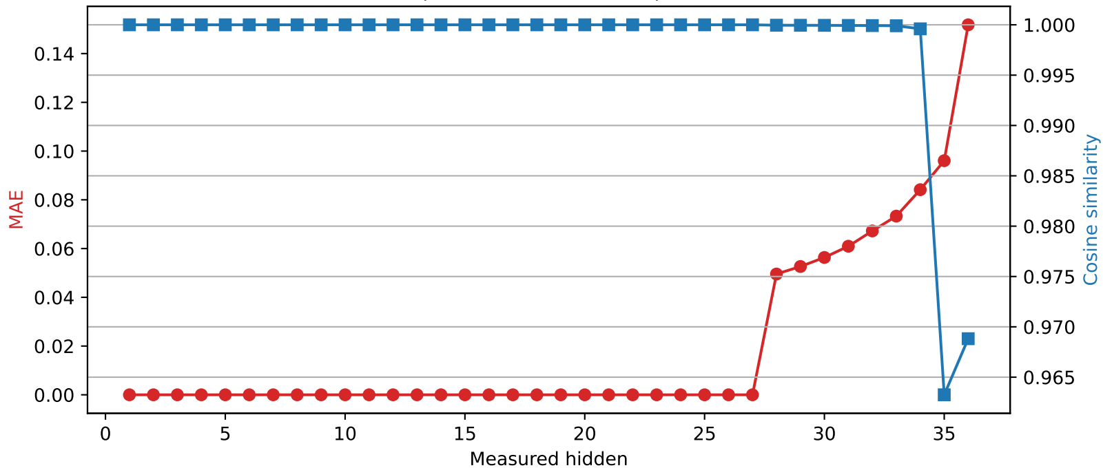
SmolLM3-3B | Quantized layer 27 | float16 → int2
