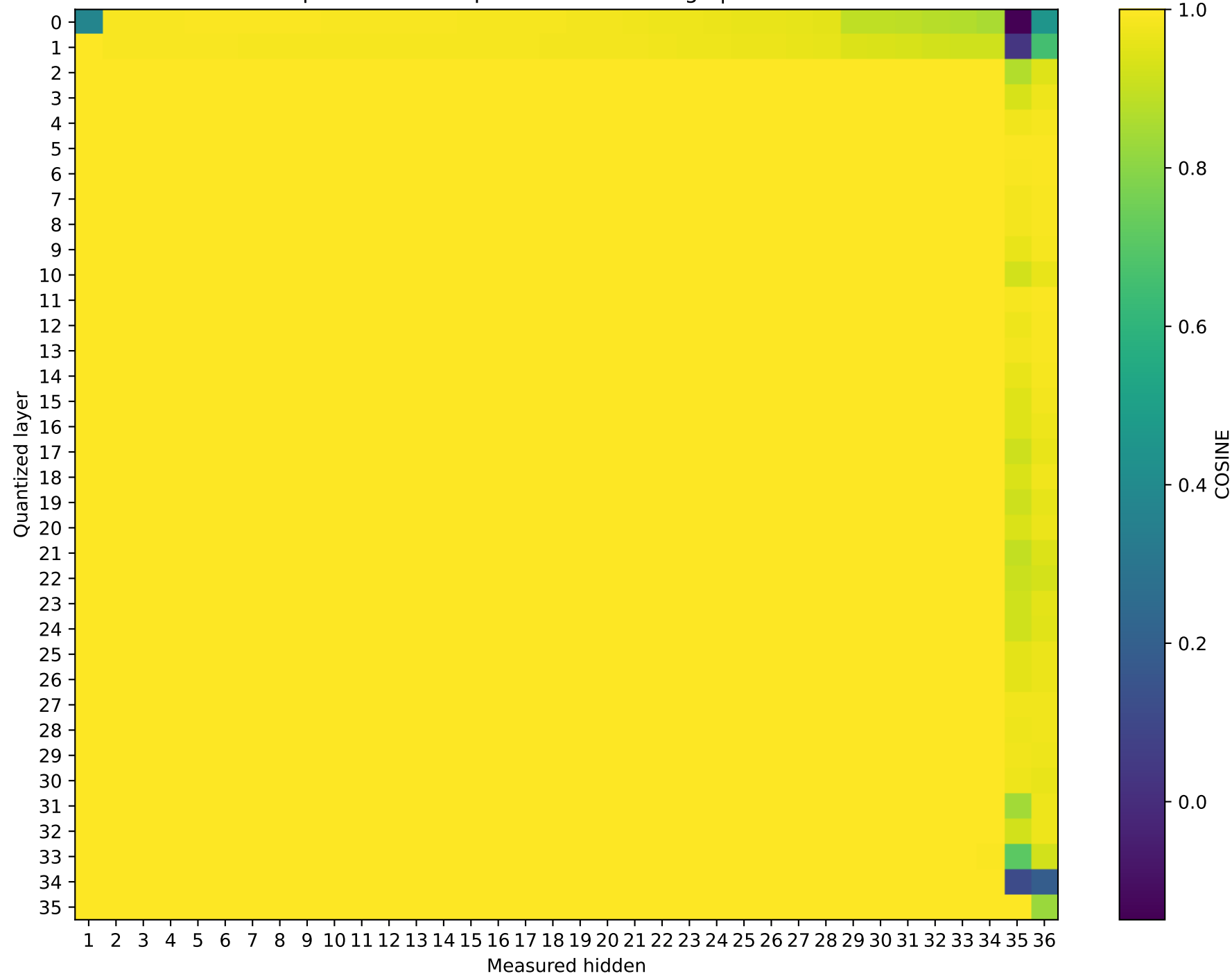
SmolLM3-3B Prompt 2: cos sim representation damage | float16 → int2
