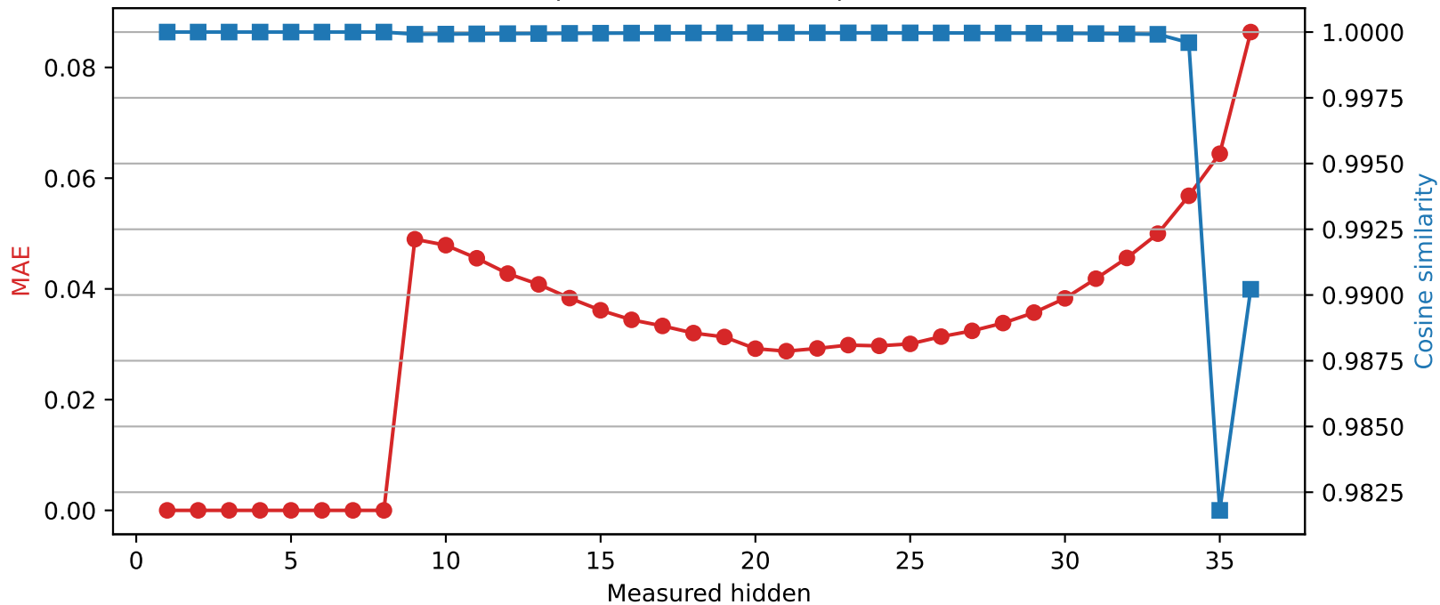
SmolLM3-3B | Quantized layer 8 | float16 → int2
