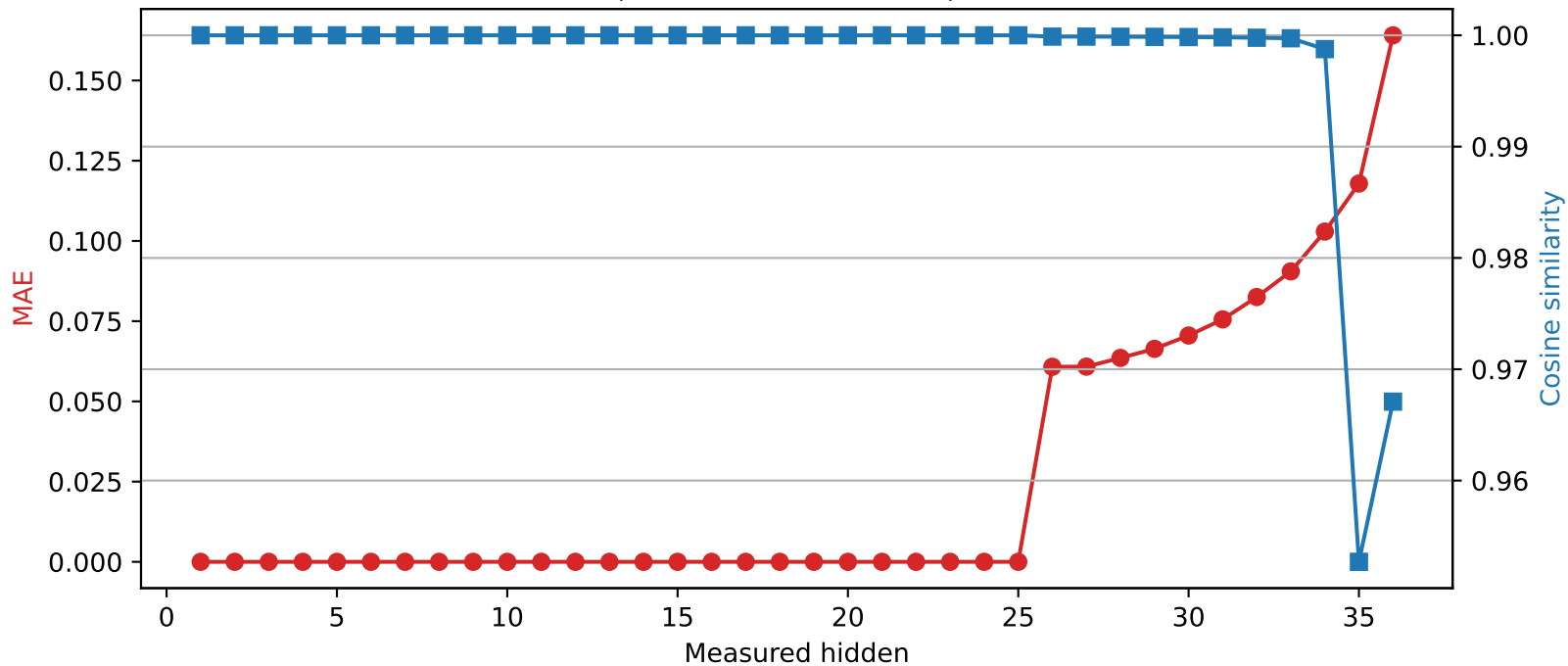
SmolLM3-3B | Quantized layer 25 | float16 \rightarrow int2
