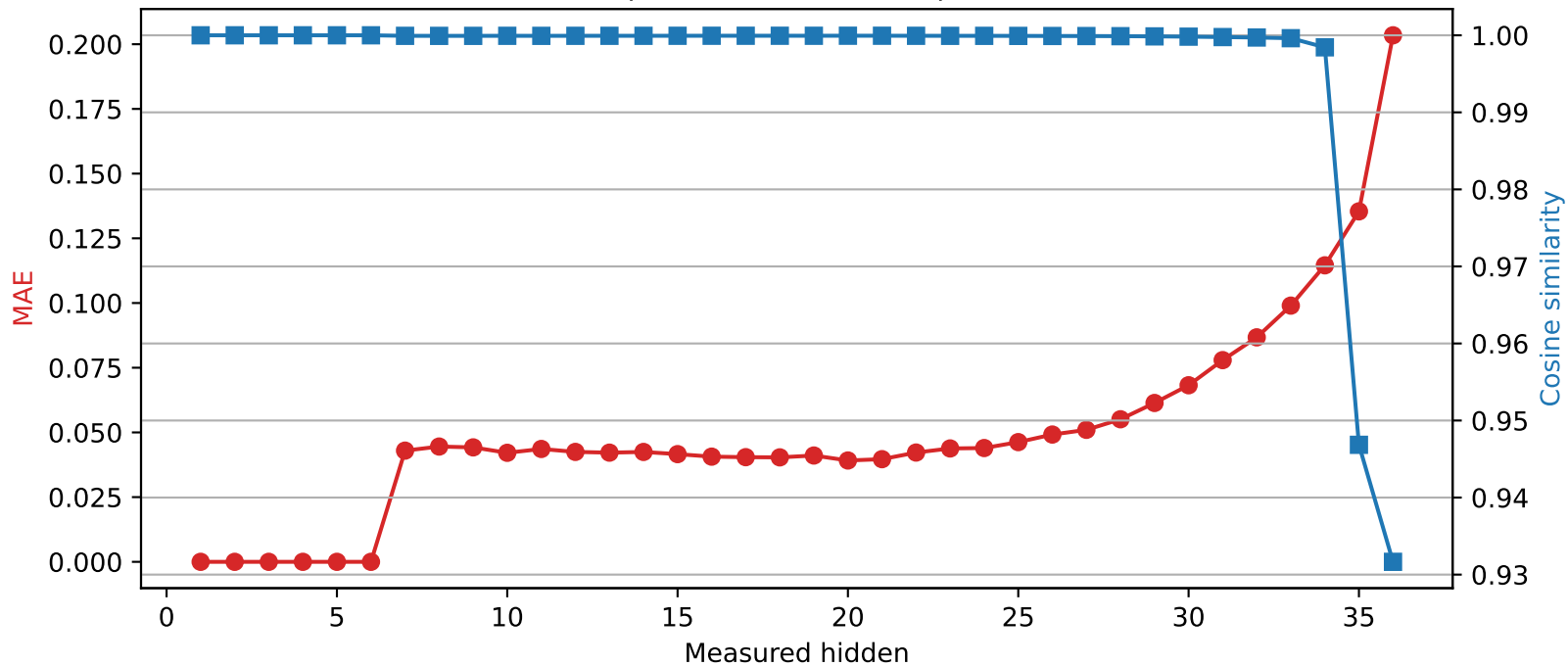
SmolLM3-3B | Quantized layer 6 | float16 \rightarrow int2
