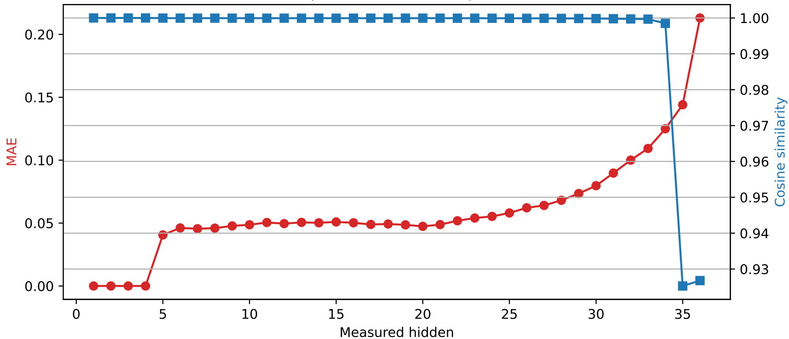
SmolLM3-3B | Quantized layer 4 | float16 → int2
