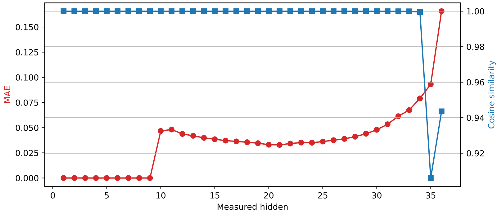
SmolLM3-3B | Quantized layer 9 | float32 → int2
