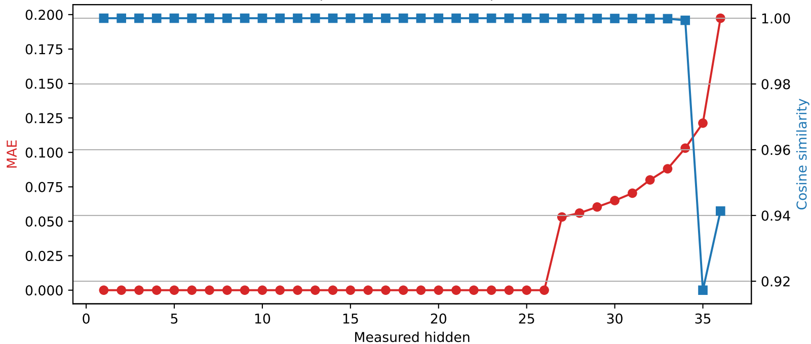
SmolLM3-3B | Quantized layer 26 | float32 → int2
