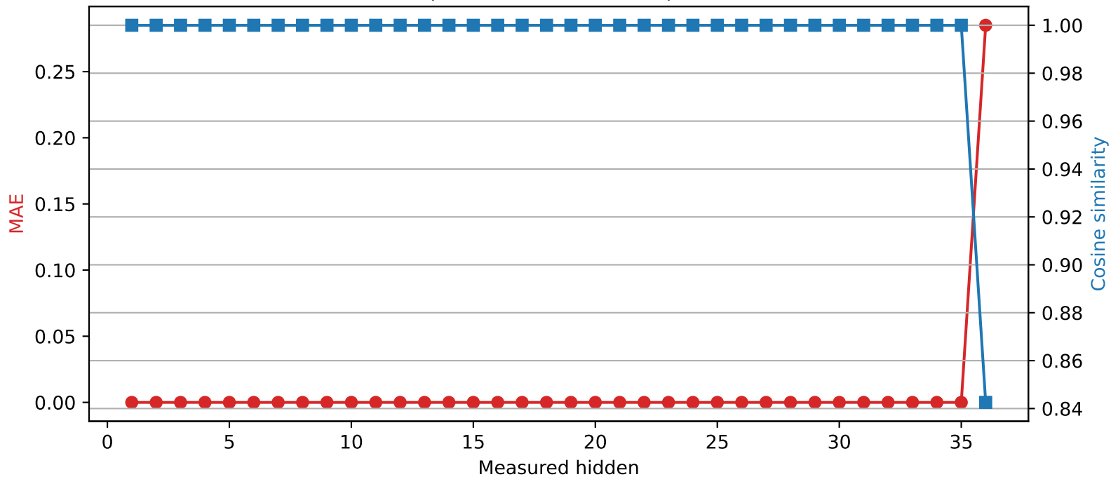
SmolLM3-3B | Quantized layer 35 | float32 \rightarrow int2
