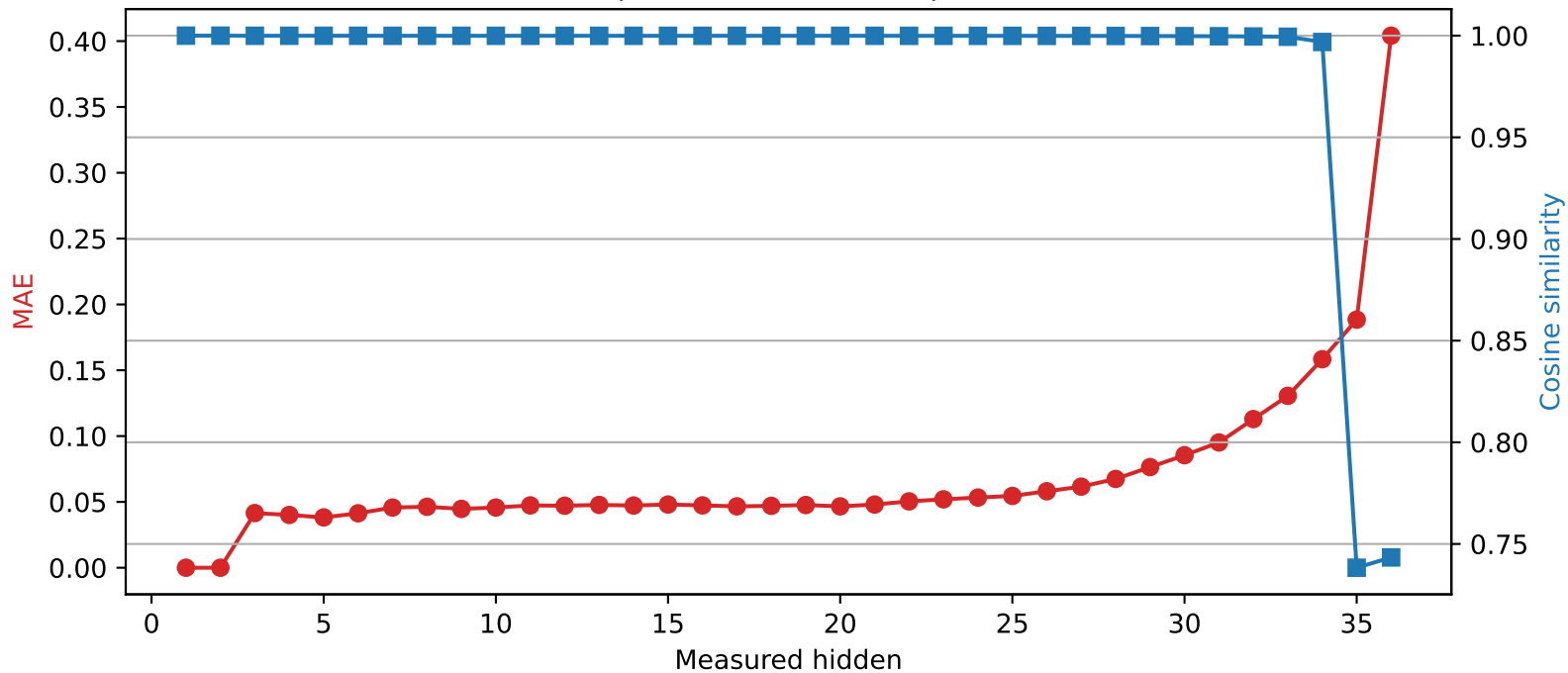
SmolLM3-3B | Quantized layer 2 | float32 → int2
