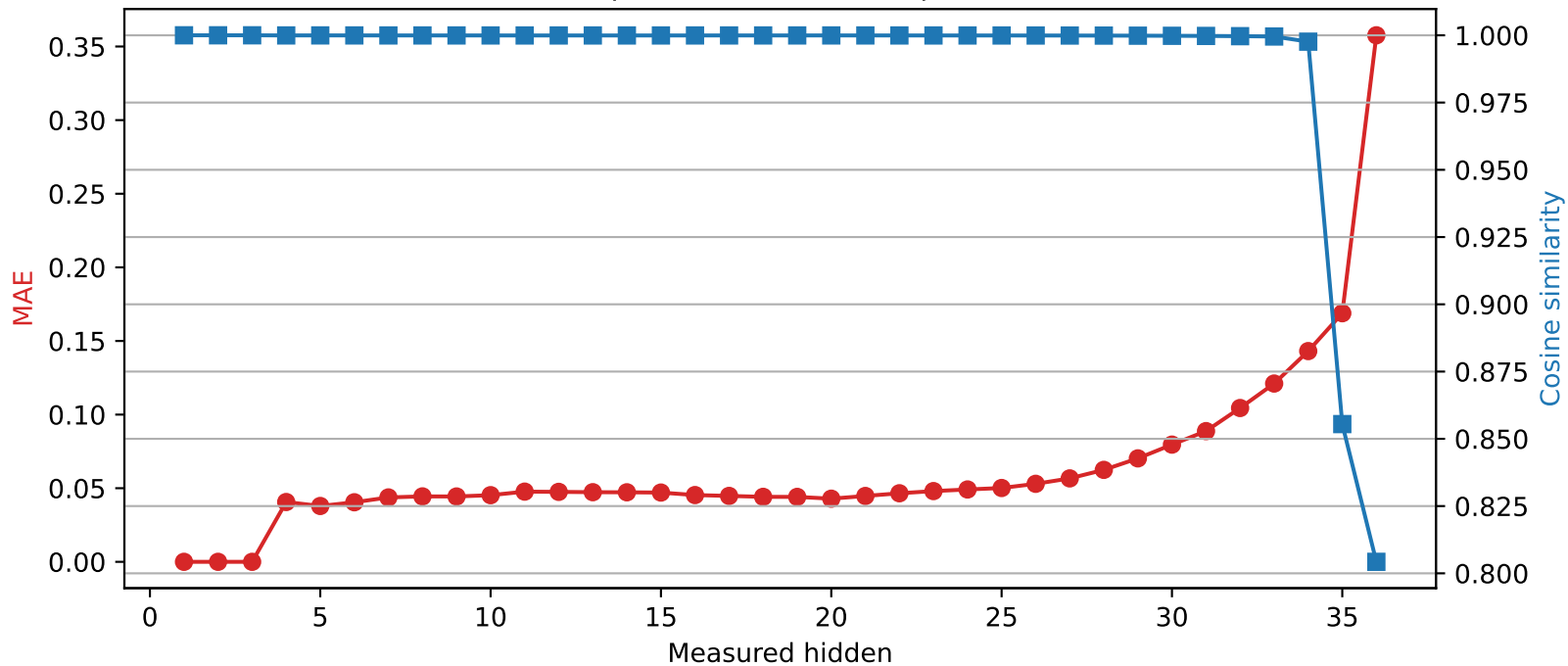
SmolLM3-3B | Quantized layer 3 | float32 \rightarrow int2
