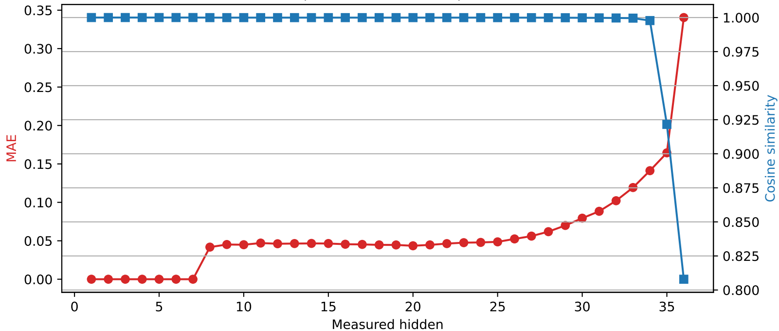
SmolLM3-3B | Quantized layer 7 | float32 → int2
