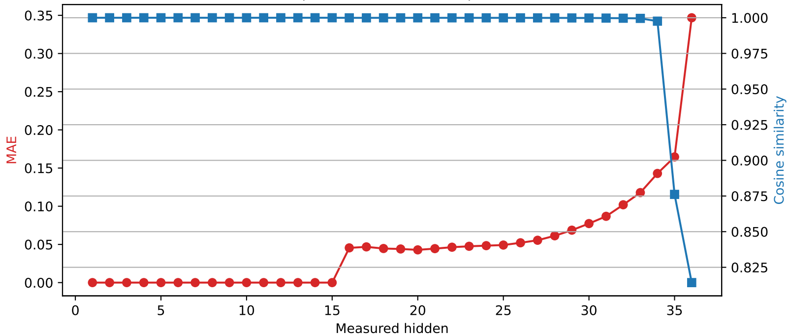
SmolLM3-3B | Quantized layer 15 | float32 \rightarrow int2
