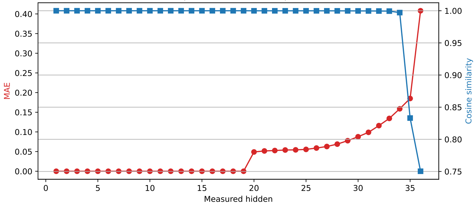
SmolLM3-3B | Quantized layer 19 | float32 \rightarrow int2
