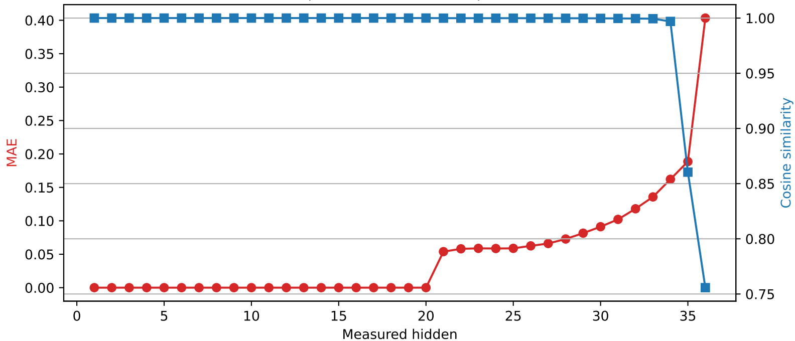
SmolLM3-3B | Quantized layer 20 | float32 → int2
