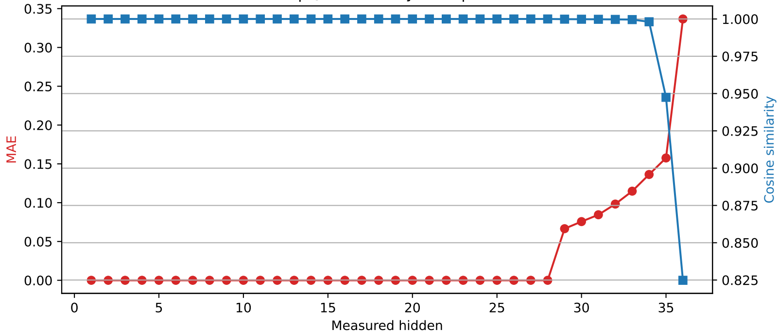
SmolLM3-3B | Quantized layer 28 | float32 → int2
