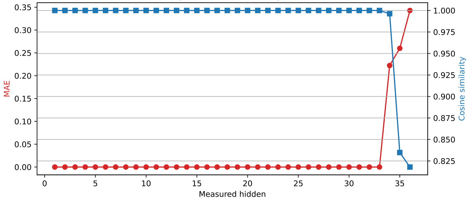
SmolLM3-3B | Quantized layer 33 | float32 → int2
