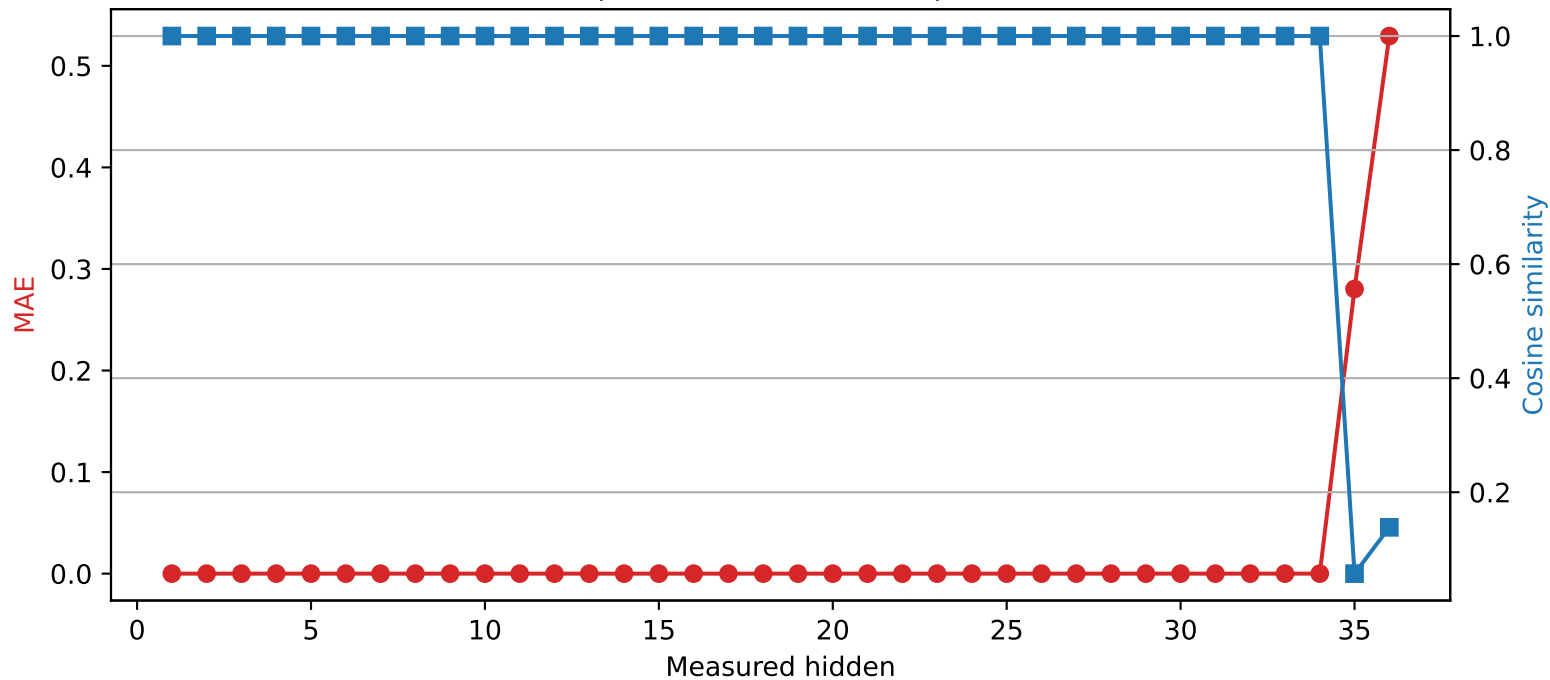
SmolLM3-3B | Quantized layer 34 | float32 → int2
