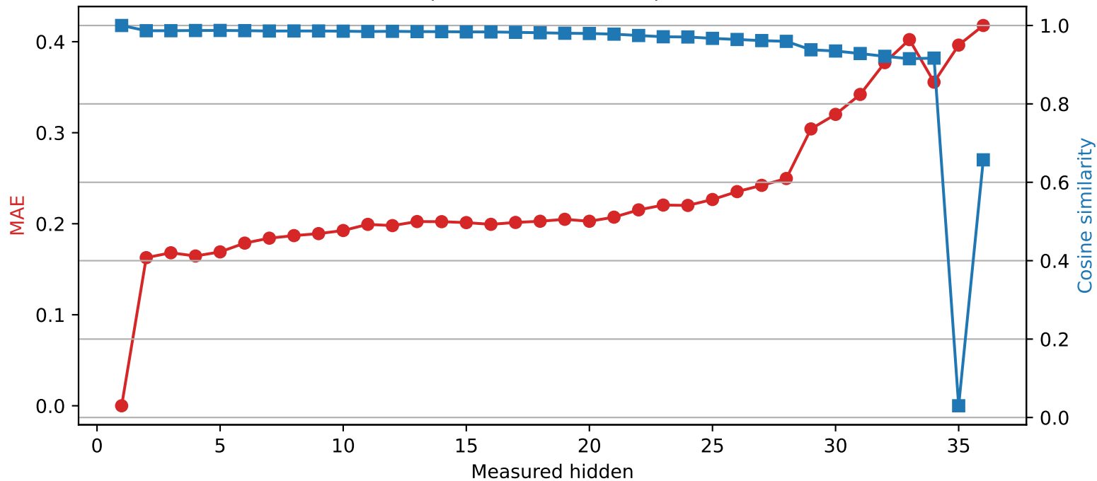
SmolLM3-3B | Quantized layer 1 | float32 \rightarrow int2
